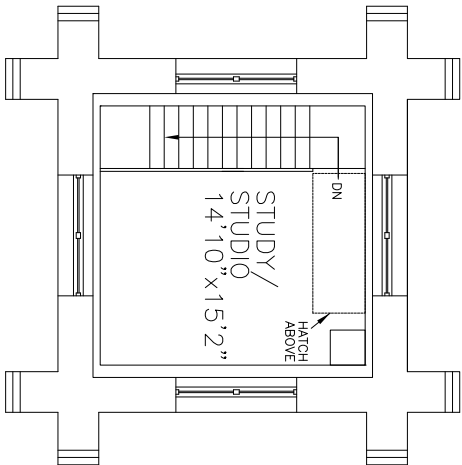
SIXTH LEVEL
