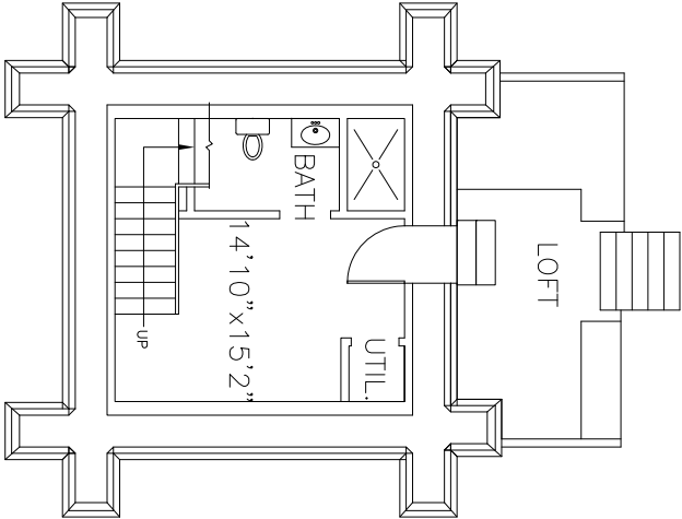
FOURTH LEVEL
