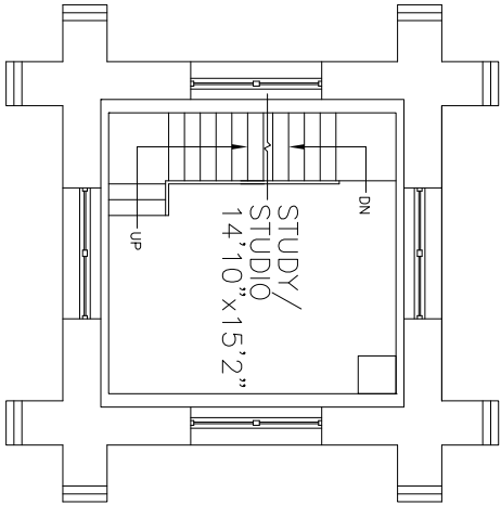
FIFTH LEVEL
